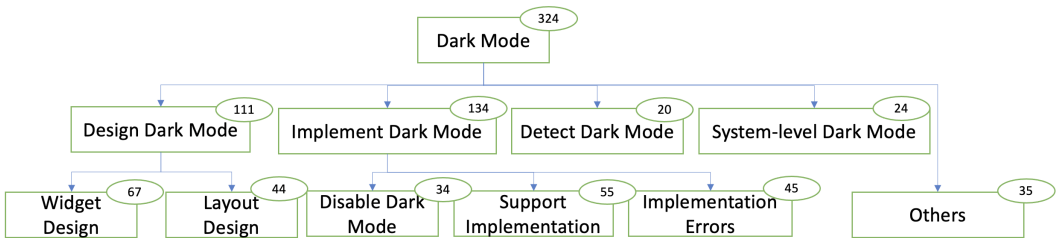
Fig. 5. Our manual classification of dark mode-related posts on Stack Overflow
