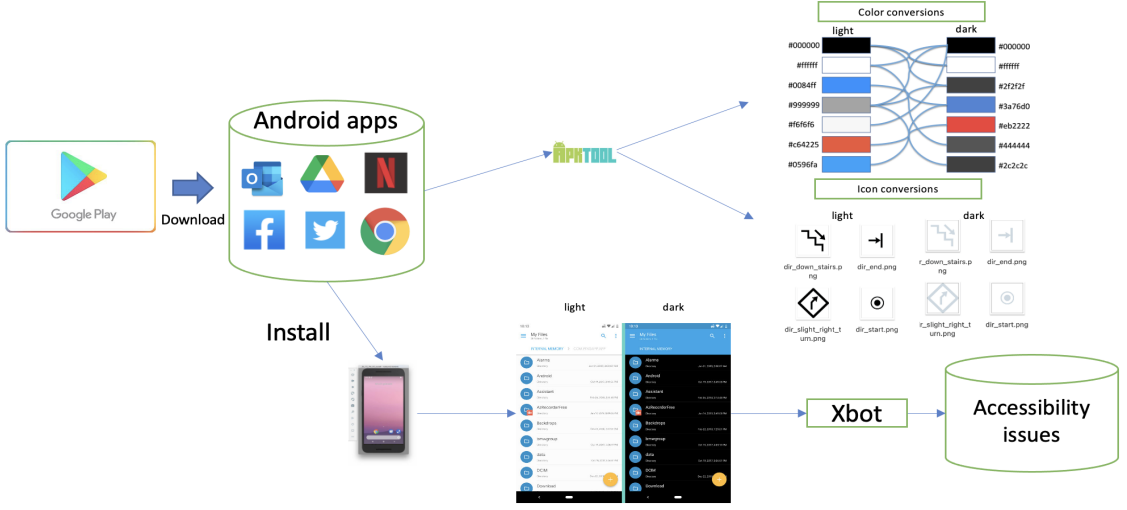
Fig. 3. Workflow of real-world Android applications analysis
